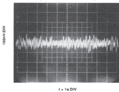
LOW FREQUENCY NOISE (0.1 Hz TO 10 Hz)
